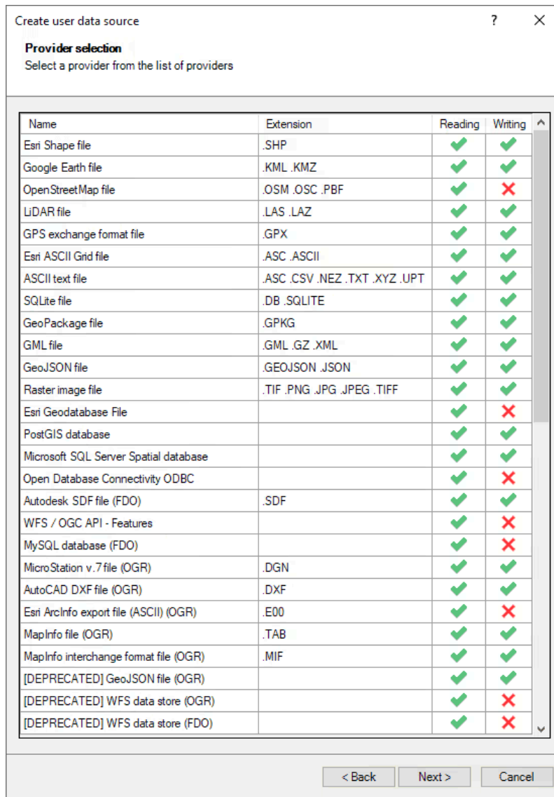
Spatial Manager™ for GstarCAD 'Create user data source' Wizard
